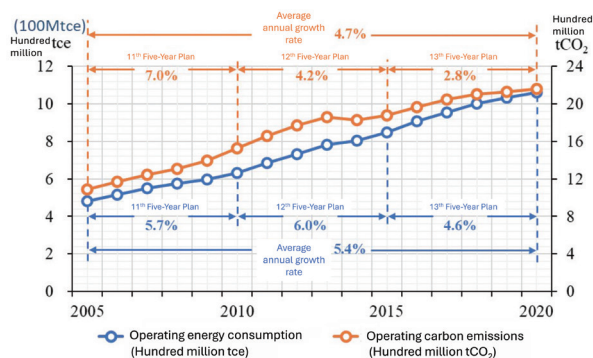
Figure 2(a) Trend of energy consumption and CO 2 emission in building operation
