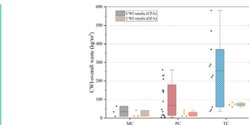
Figure 2: Construction waste reduction through using modular construction
