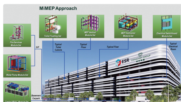
Figure 3: MiMEP Approach Adopted in the Development of Kwai Chung Cold Storage Logistic Centre
