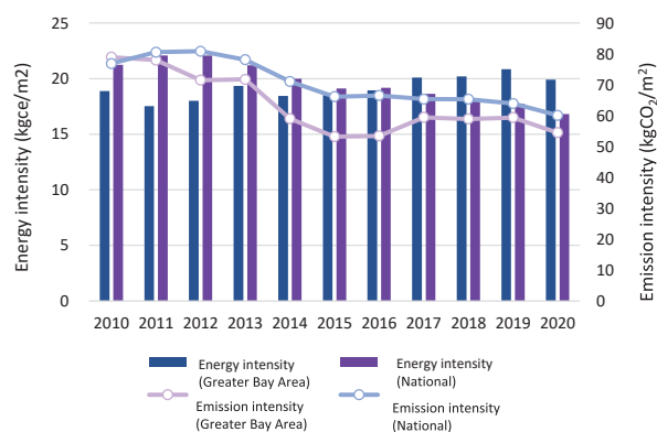
Figure 10(b) Energy intensity of non-residential buildings
